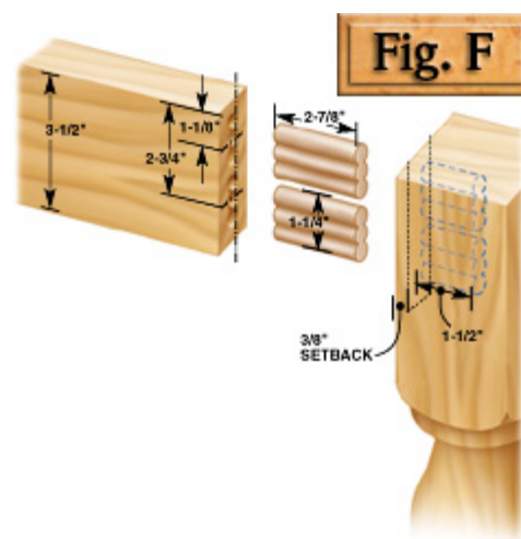
EXPLODED VIEW OF LEG AND APRON JOINERY LOOSE TENONS, cut from specially
