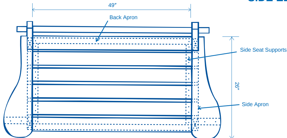
SIDE ELEVATION
