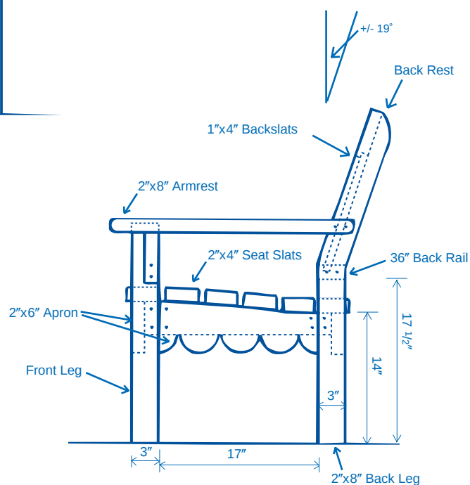
SIDE ELEVATION
