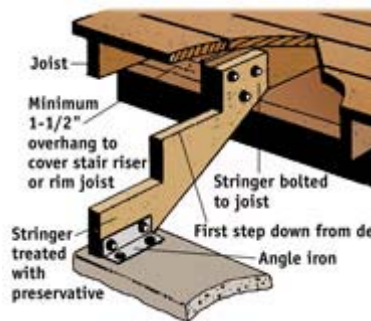
FIG. 7 - The stringer can be bolted to the end of the joist so the first step is one step below the surface of the deck. At the landing pad, the stringer may be fastened to an angle iron (the angle should be galvanized) bolted to the concrete. From the Sunset book, Decks, © Sunset Publishing Corporation.
