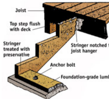
FIG. 6 - Stringers may be hung from the rim joist with a joist hanger so the first step is flush with the deck surface. In this configuration, a piece of pressure-treated lumber is bolted to the landing pad and the stringer is nailed to it with 16d galvanized nails. From the Sunset book, Decks, © Sunset Publishing Corporation.
