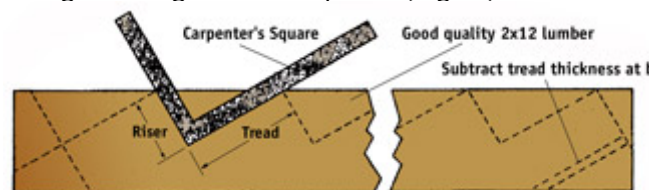
FIG. 5 - Set the carpenter's square on the stringer so the riser and tread dimensions are at the edge, then trace along the square. Move the square to the previous mark and repeat the process. Subtract one tread thickness from the layout at the bottom so the last step is equal in height to the rest. From the Sunset book, Decks, © Sunset Publishing Corporation.
