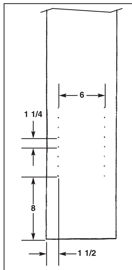
Figure 6 Hole Pattern Diagram (Boards D and H)
