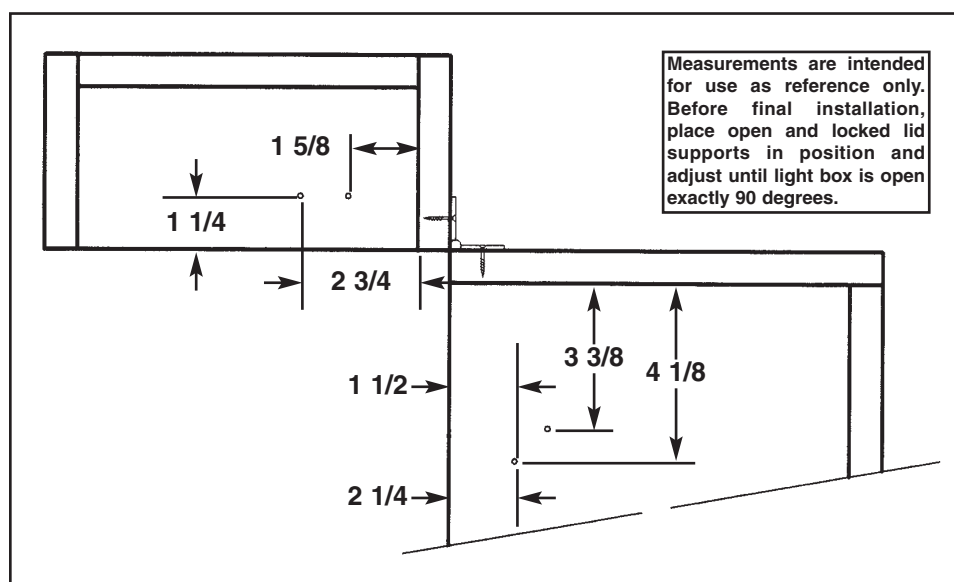
Figure 7 Lid Support Installation Guide
