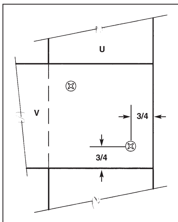
Figure 8 Leg Screw Locations
