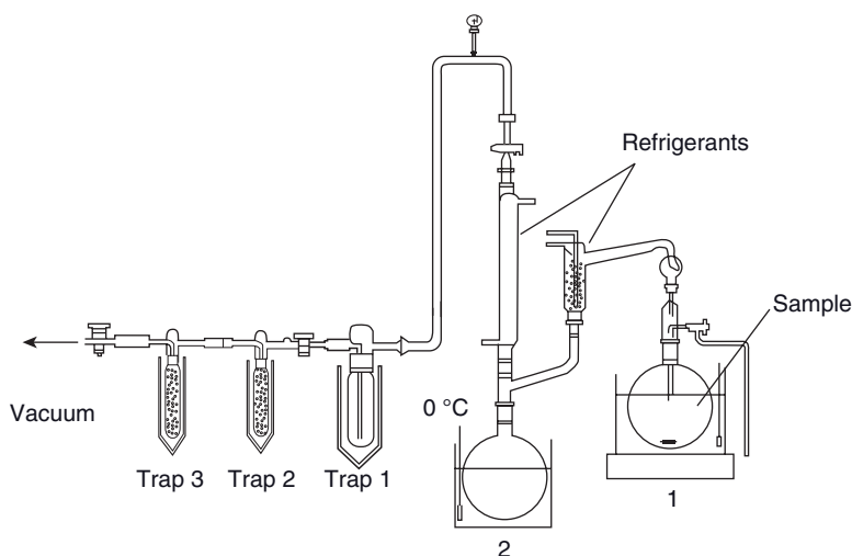
Figure 33.3. Apparatus for vacuum distillation proposed by Forss and Holloway (1967).
