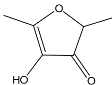
Figure 21.1. Furaneol (2,5-dimethyl-4-hydroxy-3(2H)-furanone).
