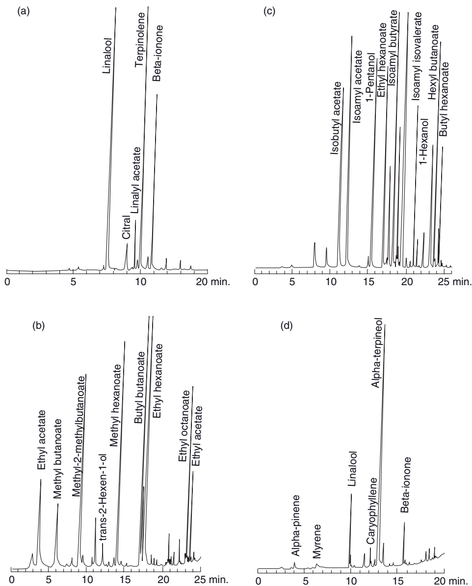
Figure 13.7. Gas chromatographic patterns of the SPME extracts of (A) raspberry, (B) strawberry, (C) banana, and (D) mango. SPME conditions: fiber, 100 \mu m PDMS; extraction mode, headspace; sample, solid (1 g); extraction, 60°C for 30 min; desorption, 200°C for 15 min. GC conditions: column, CP-Sil-5CB (50 m \times 0.25 mm i.d., 0.25- \mu m film thickness); column temperature, program from 50°C (3-min hold) to 250°C at 5°C/min and hold at 250°C for 17 min; injection temperature, 200°C; detector temperature, 250°C; detection, flame ionization detector (FID). Reproduced from Ibanez and others (1998).
