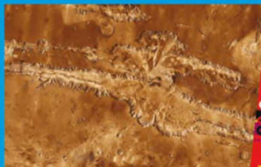
Valles Marineris is the biggest canyon in the Solar System
