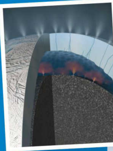
Large geysers of water vapour fire out from the south pole of Enceladus
