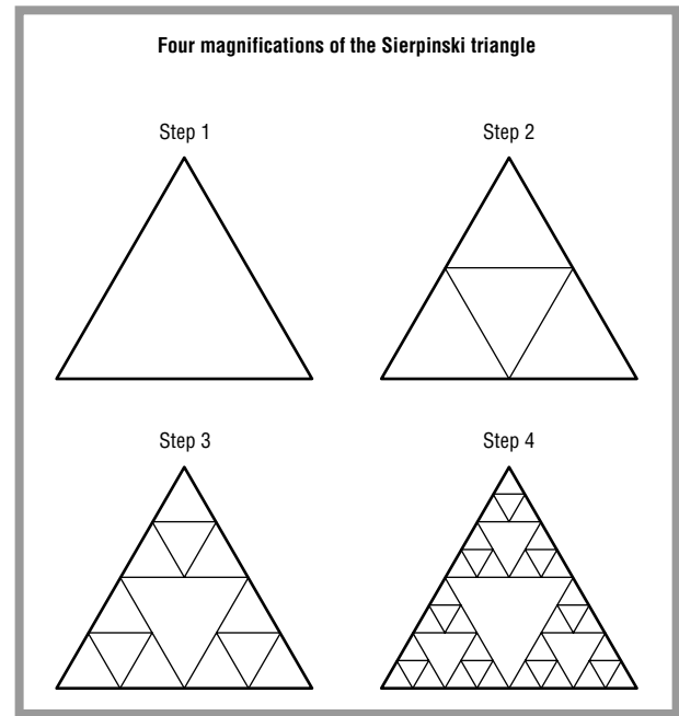
Figure 5: Sierpinski triangles.
